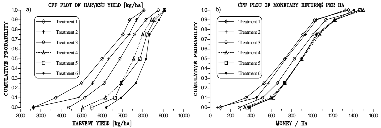
Fig. 5. Cumulative probability function plots of the simulated harvest maize yield (a) and monetary returns (b) in Kojnare under 2xCO 2 CCC climate change scenario.
