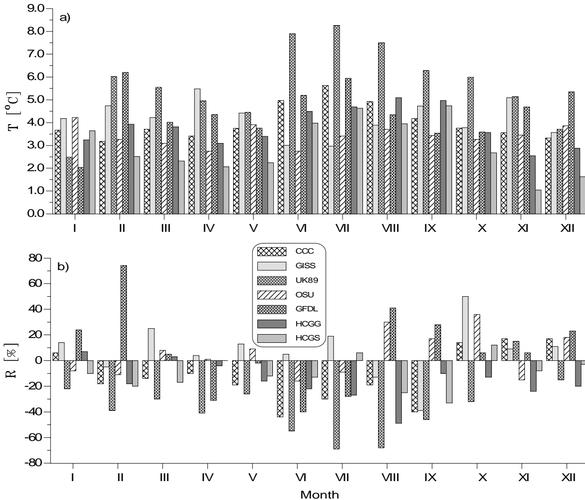
Fig. 3. Climate change scenarios for Bulgaria - differences/ratios between 2xCO 2 and 1xCO 2 GCM outputs for monthly air temperature (a) and precipitation (b).
